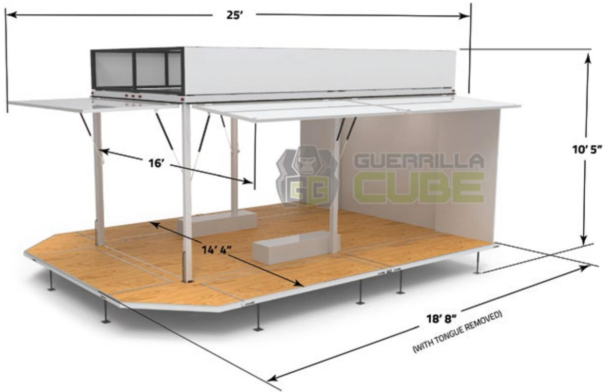
SPLIT DOOR, WITH CORNER FILLERS AND WALK ON ROOF, OPEN
