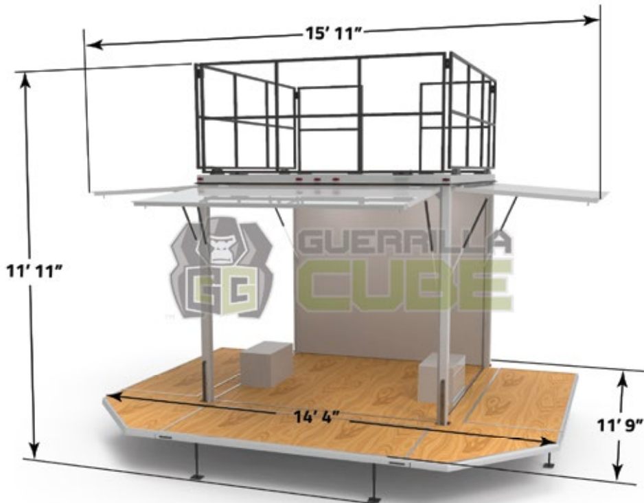
SPLIT DOOR, WITH CORNER FILLERS AND ROOF RAILINGS, OPEN
